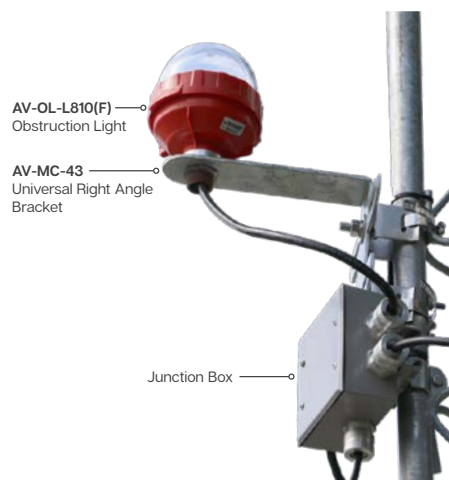
E-1 Kit installation showing the Universal Right Angle Bracket (AV-MC-43) with an L-810(F) single fixture obstruction light.
