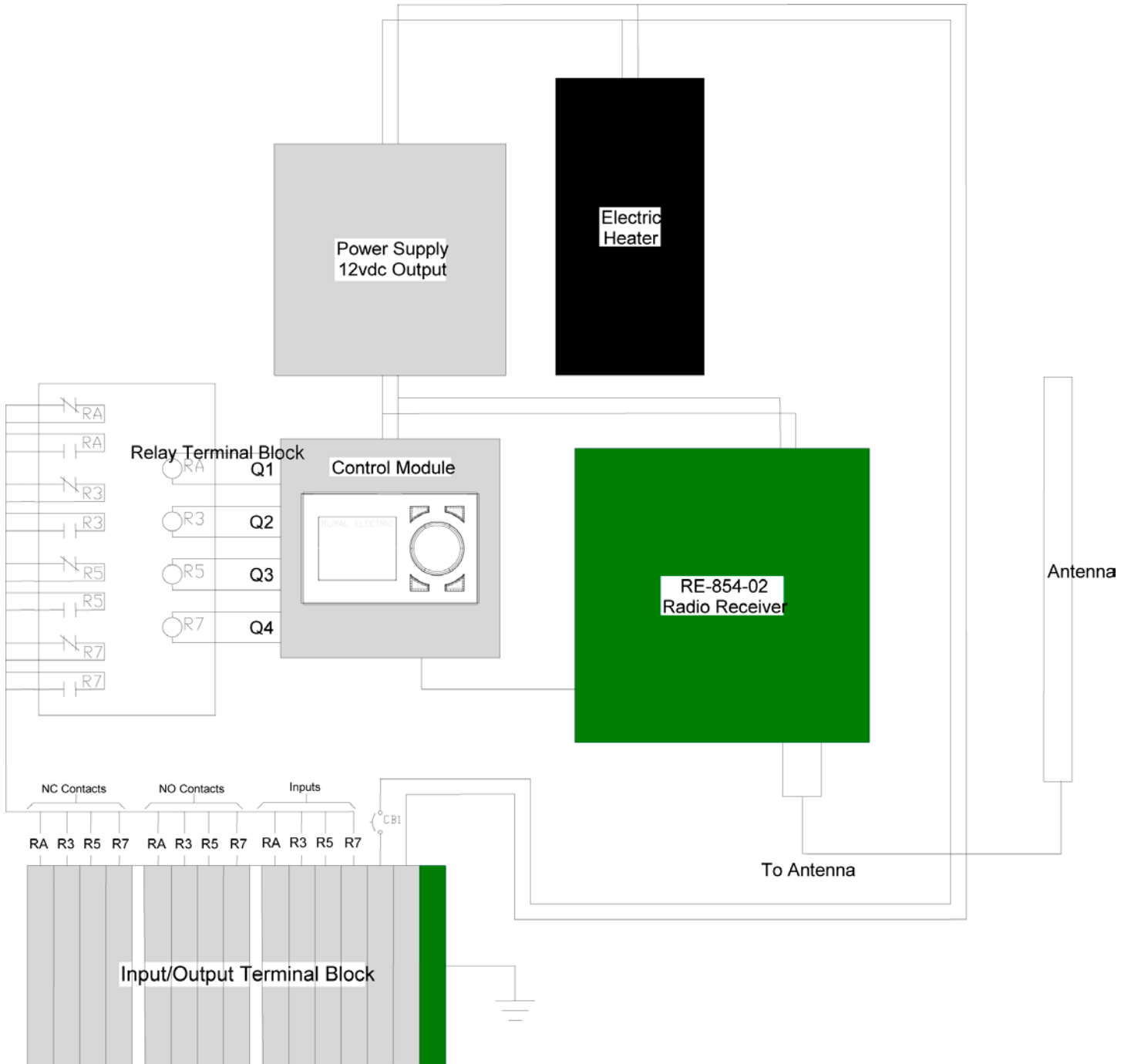
Component Layout
