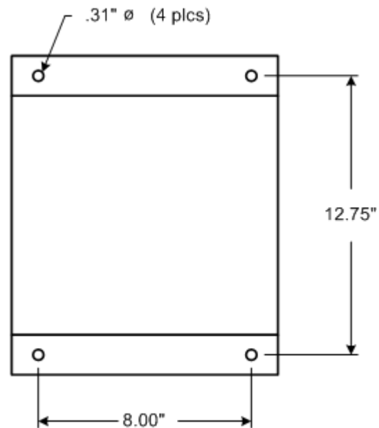
Mounting Layout
